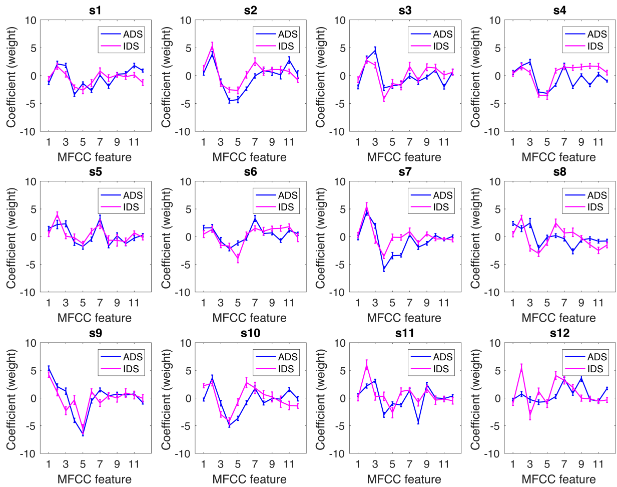
Figure S1. Average MFCC feature vectors across all utterances for each English-speaking participant; related to Figure 1. Each plot represents data from one participant’s adult-directed and infant-directed speech. N = 12. Error bars represent \pm SEM across 20 utterances.
